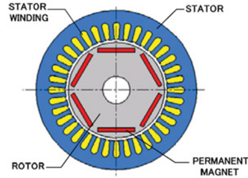
IPM Motor
