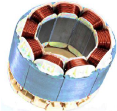
Concentrated Winding with segmented stator construction
