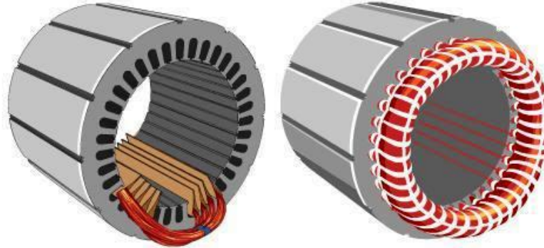
Distributed Winding
