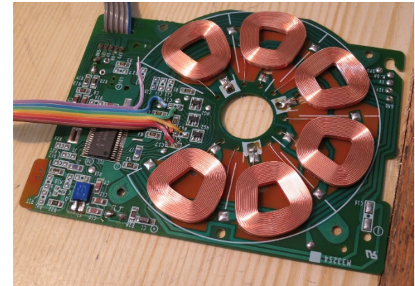
Slotless axial air gap winding
