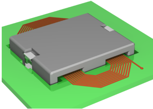
Planar transformer
