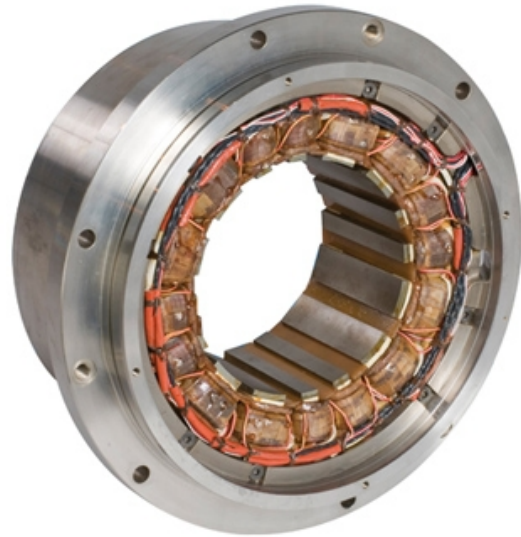
Electromagnetic bearing
