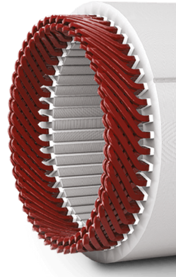
Copper bar winding
