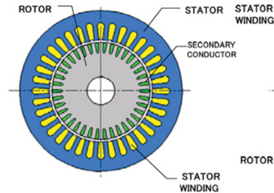
Induction Motor
